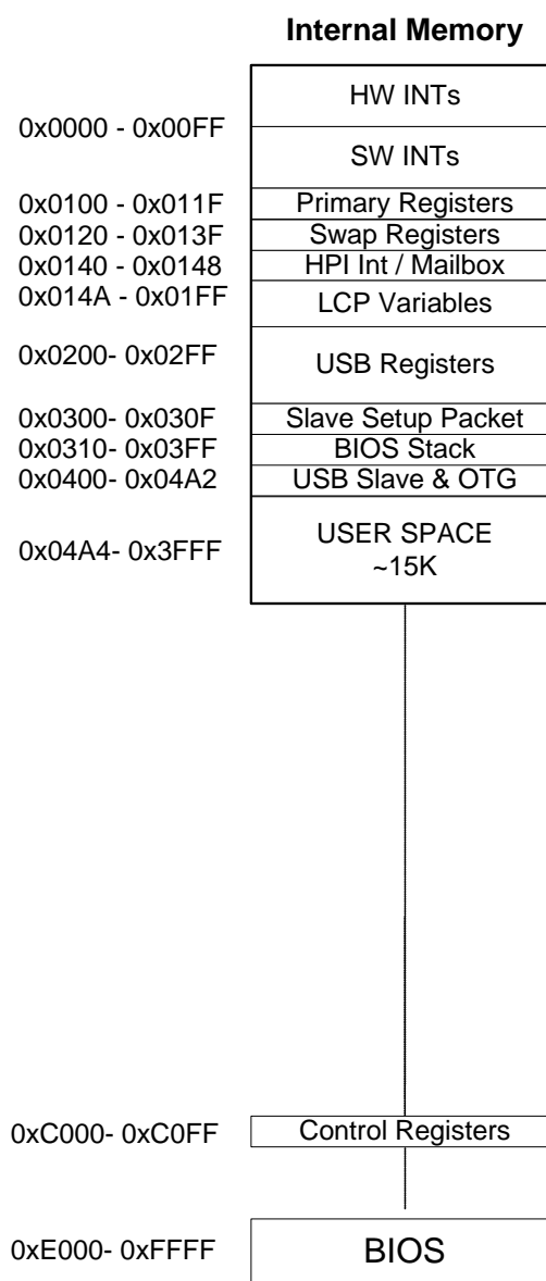
Figure 6. Memory Map
