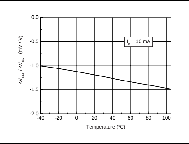
Figure 15. Ratio of change in V_{REF} to change in V_{KA} vs. temperature
