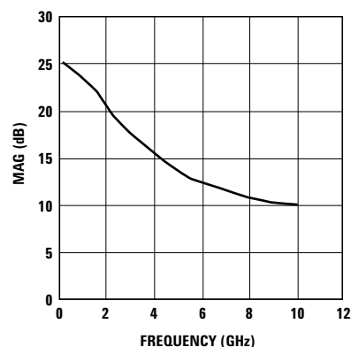
Figure 32. MAG vs. Frequency.
