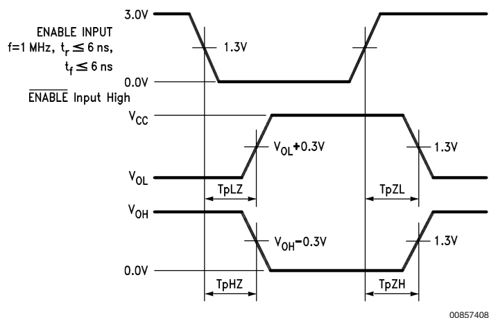
FIGURE 6. Enable and Disable Times for “LS-Type” Load
