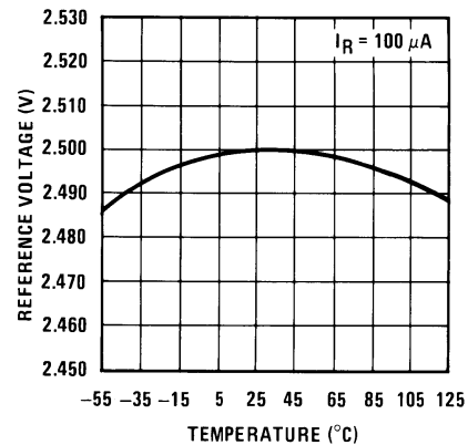
Temperature Drift
