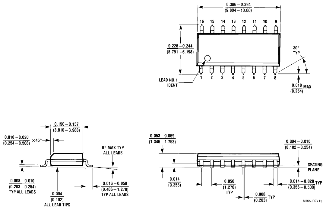
16-Lead Molded Small Outline Package (M) Order Number DS34C86TM NS Package Number M16A
