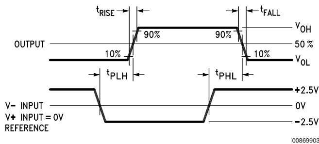
FIGURE 1. Propagation Delays
