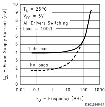
Power Supply Current vs Frequency
