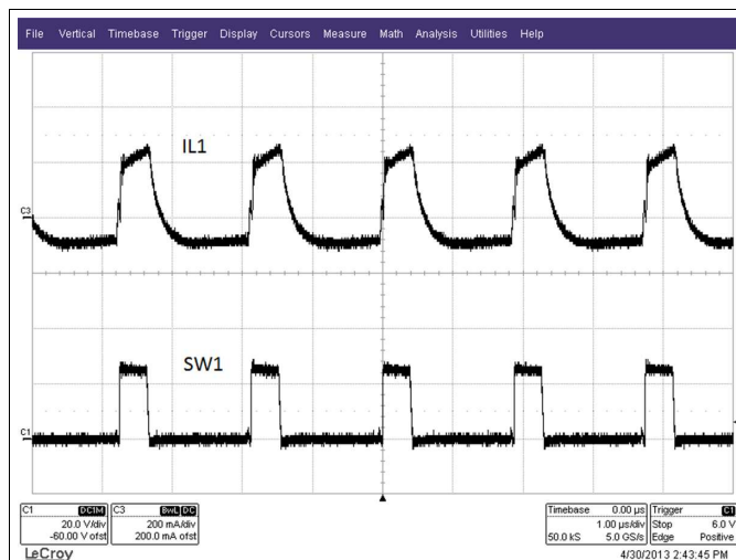
Figure 21. Steady State Waveform ( V_{IN} = 24 V , I_{OUT1} = 0 mA , I_{OUT2} = 200 mA )
