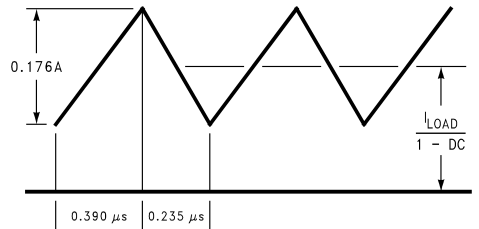
Figure 30. 10 μH Inductor Current, 5V–12V Boost (LM2731X)
