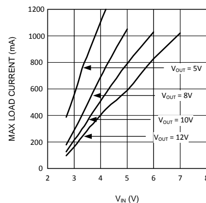
Figure 34. Max. Load Current (typ) vs V IN - "Y"
