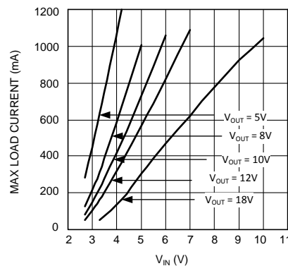
Figure 33. Max. Load Current (typ) vs V IN - "X"
