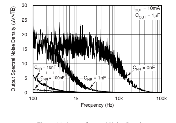
Figure 24. Output Spectral Noise Density vs Noise Reduction
