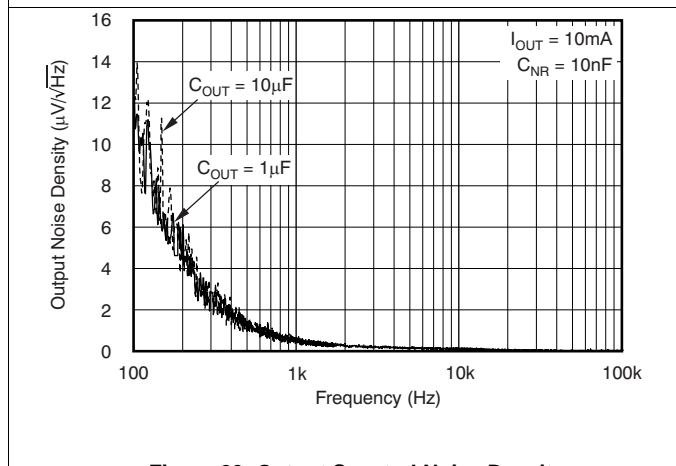
Figure 23. Output Spectral Noise Density vs Output Capacitance
