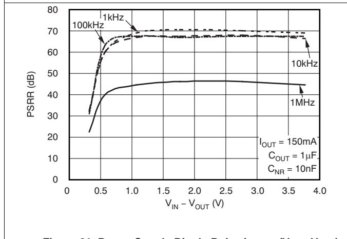
Figure 21. Power-Supply Ripple Rejection vs ( V_{IN} - V_{OUT} )
