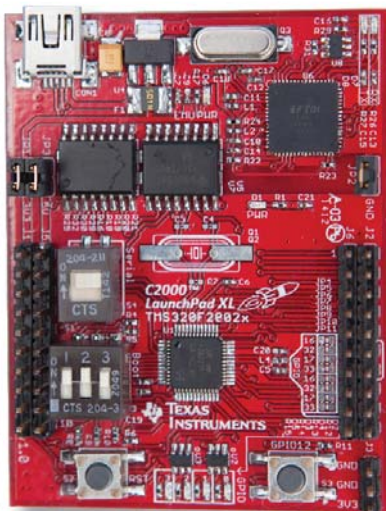
▲ C2000 LaunchPad (shown at actual size of 2.0" x 2.6")
