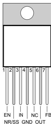
KC PACKAGE TO-220-7 (Top View)
