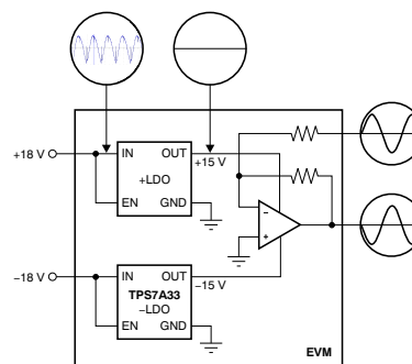
Typical Application: Post DC/DC Converter Regulation for High-Performance Analog Circuitry
