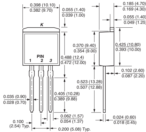
TO-262AA
