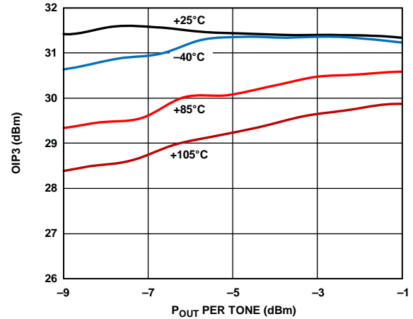
Figure 38. OIP3 vs. POUT at 30 MHz
