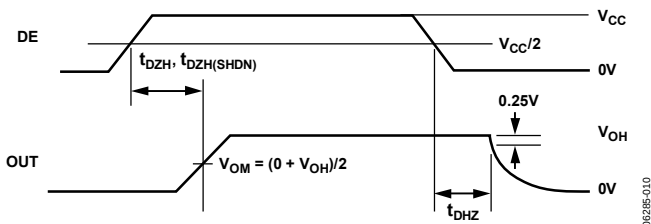
Figure 10. Driver Enable and Disable Times ( t_{DZH} , t_{DZH(SHDN)} , t_{DHZ} , t_{DHZ(SHDN)} )
