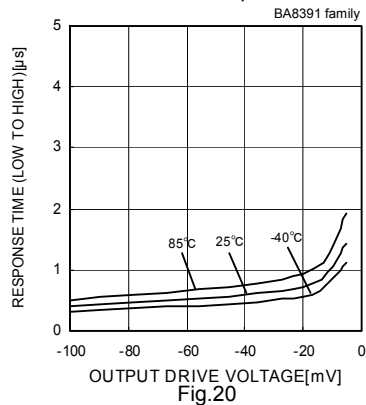
Response Time (Low to High) - Over Drive Voltage (VCC=5[V],VRL=5[V],RL=5.1[kΩ])
