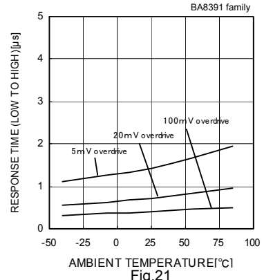
Response Time (Low to High) - Ambient Temperature (VCC=5[V],VRL=5[V],RL=5.1[kΩ])
