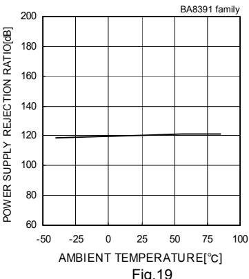
Power Supply Rejection Ratio - Ambient Temperature
