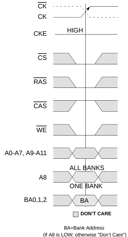
PRECHARGE Command
