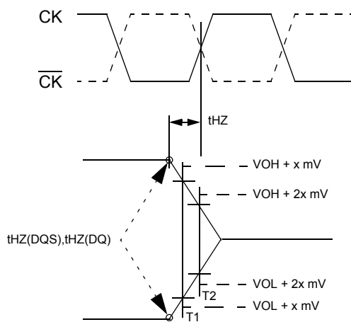
Figure 55. tLZ and tHZ method for calculating transitions and endpoints
