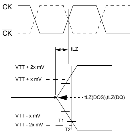
Figure 55. tLZ and tHZ method for calculating transitions and endpoints
