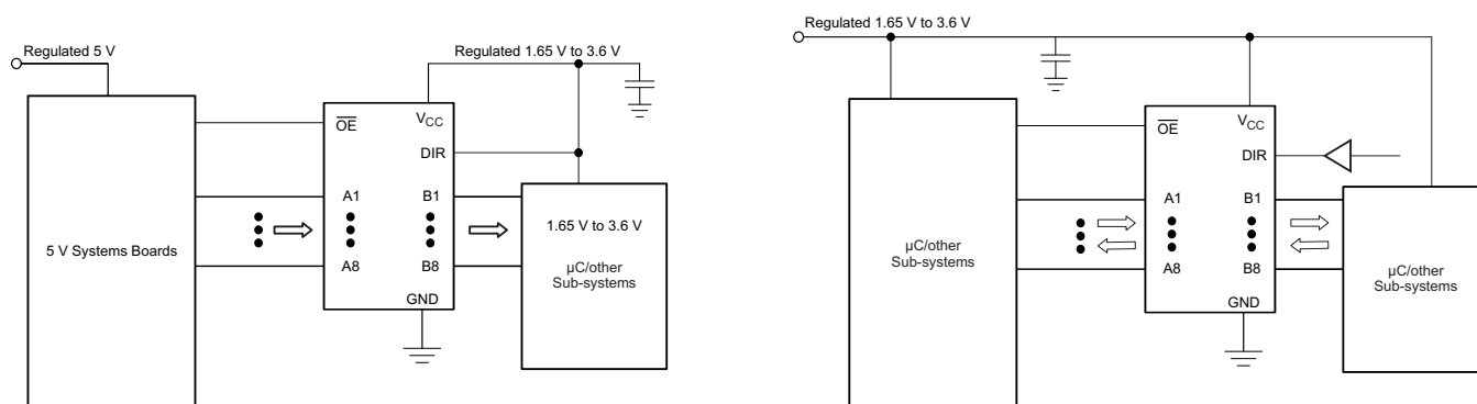
Figure 4. Typical Application Diagram
