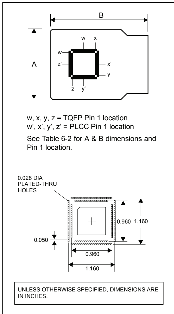
FIGURE 6-3: DVA DRAWING – DOUBLE-ROW TQFP/PLCC
