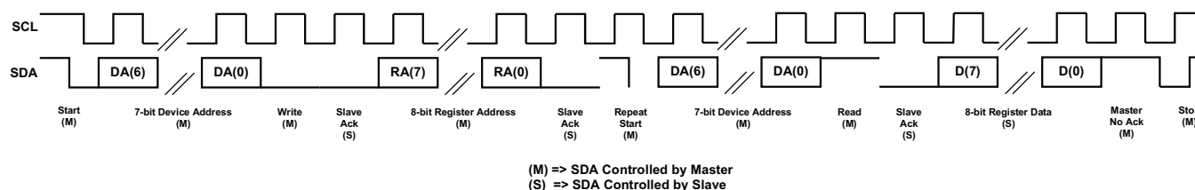
Figure 17. I²C Read
