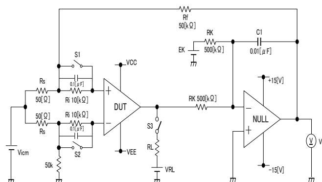
Fig.88 Measurement circuit1 (one channel only)
