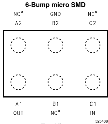
Top View (Bump Side Down)
