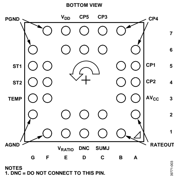
Figure 3. Pin Configuration
