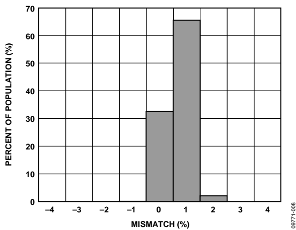
Figure 12. Self-Test Mismatch at 25°C ( V_{RATIO} = 5 V )
