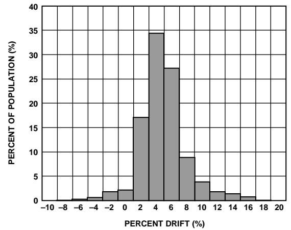
Figure 8. Sensitivity Drift over Temperature
