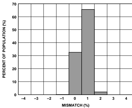
Figure 12. Self-Test Mismatch at 25°C
