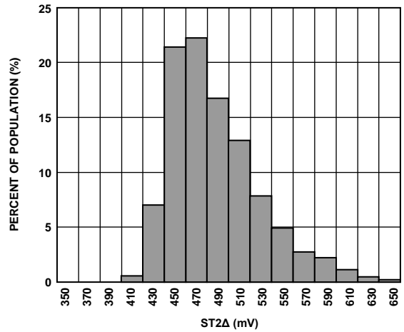
Figure 13. ST2 Output Change at 25°C
