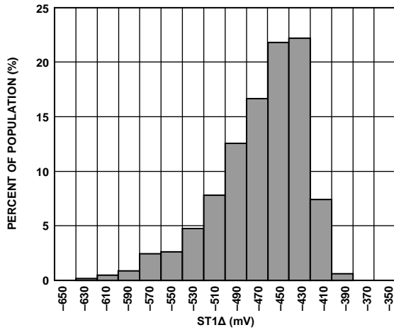
Figure 10. ST1 Output Change at 25°C
