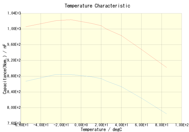
C1608X5R1A105K080AC(DC Bias = 0V) C1608X5R1A105K080AC(DC Bias = 5V)
