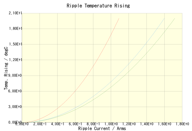
C1608X5R1A105K080AC(100kHz) C1608X5R1A105K080AC(500kHz) C1608X5R1A105K080AC(1MHz)
