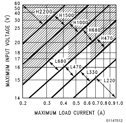
FIGURE 5. LM2575(HV)-12
