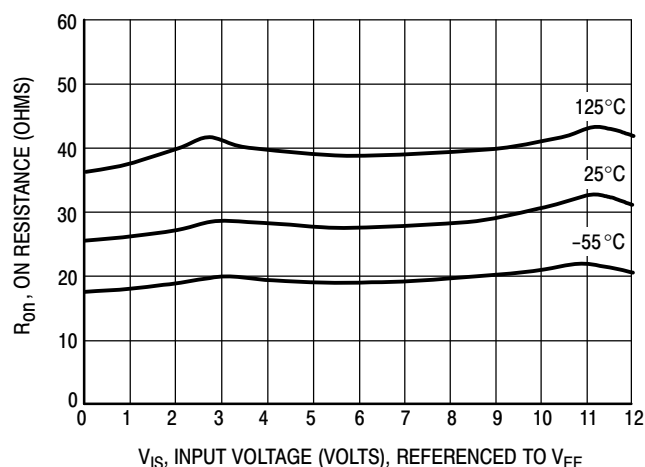
Figure 1f. Typical On Resistance, V_{CC} - V_{EE} = 12.0 \text{ V}
