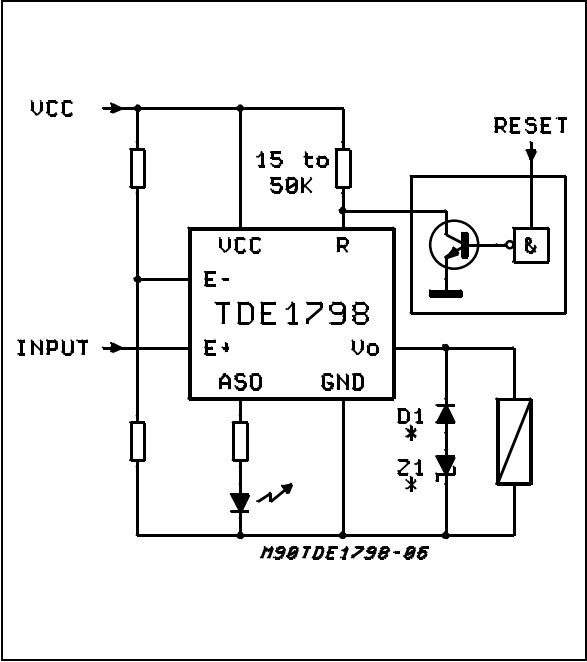
TYPICAL APPLICATION CONTROLLED RESET
