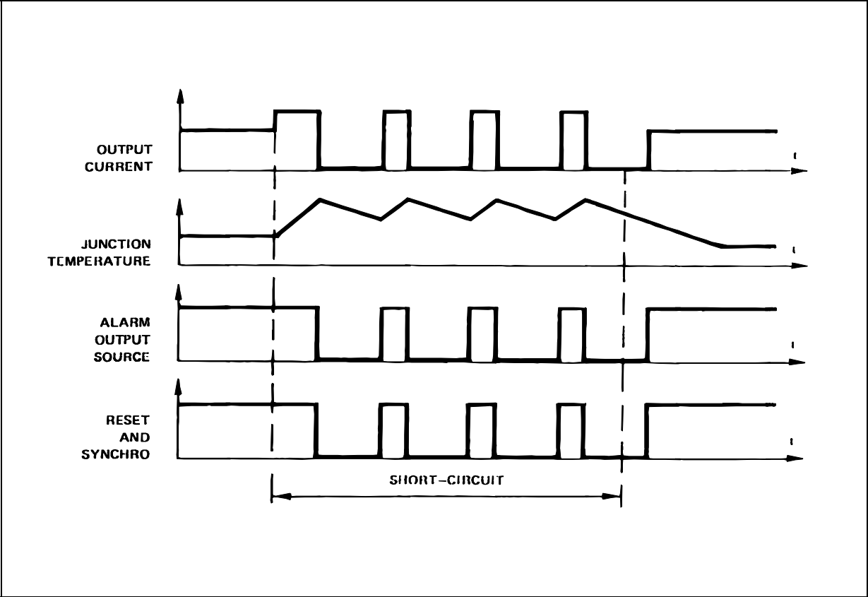
SHORT CIRCUIT CONDITIONS WITH AUTOMATIC RESET
