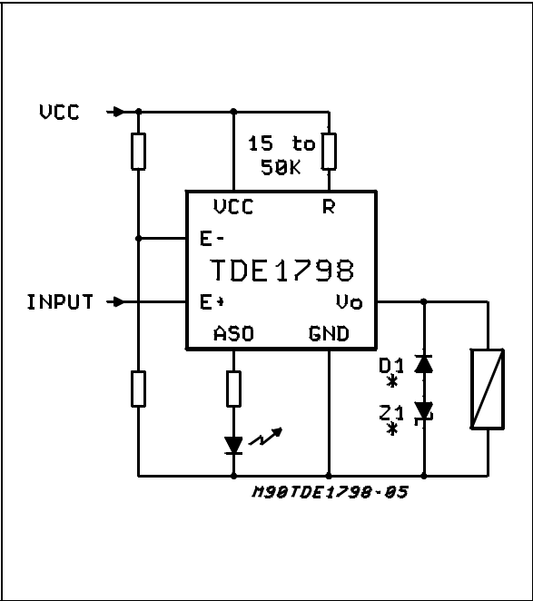
TYPICAL APPLICATION AUTOMATIC RESET
