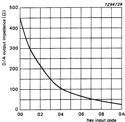
(a) Output impedance near negative power rail; T_{amb} = +27^\circ C .
