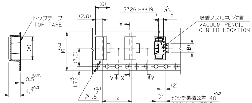
SECT:X-X
