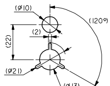
DETAIL F
