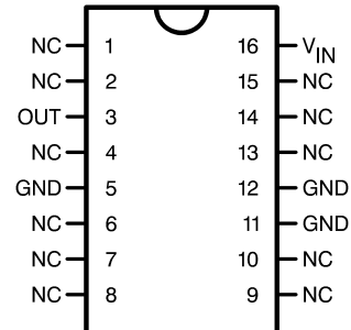
Top View See NS Package Number WG16A
