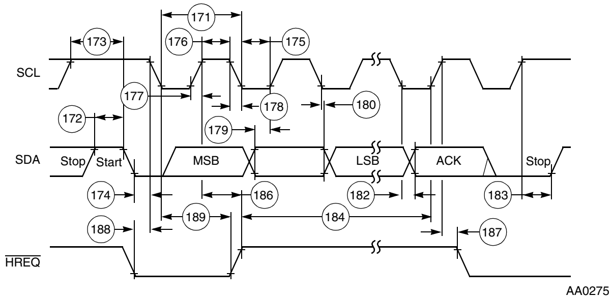
Figure 3-31 I²C Timing
