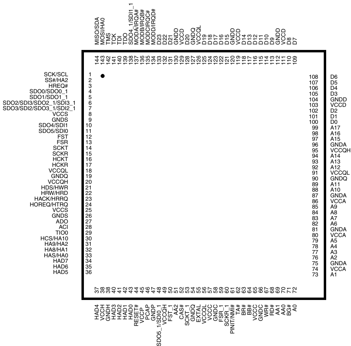
Figure 4-1 144-pin package
