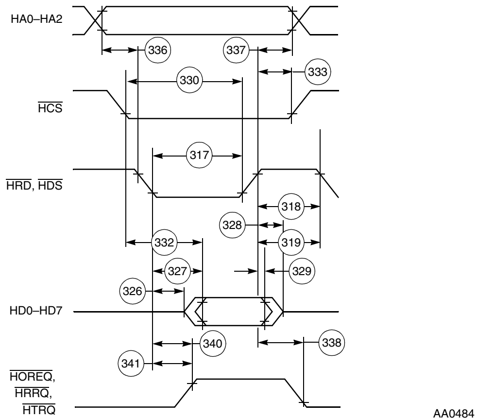
Figure 3-21 Read Timing Diagram, Non-Multiplexed Bus
