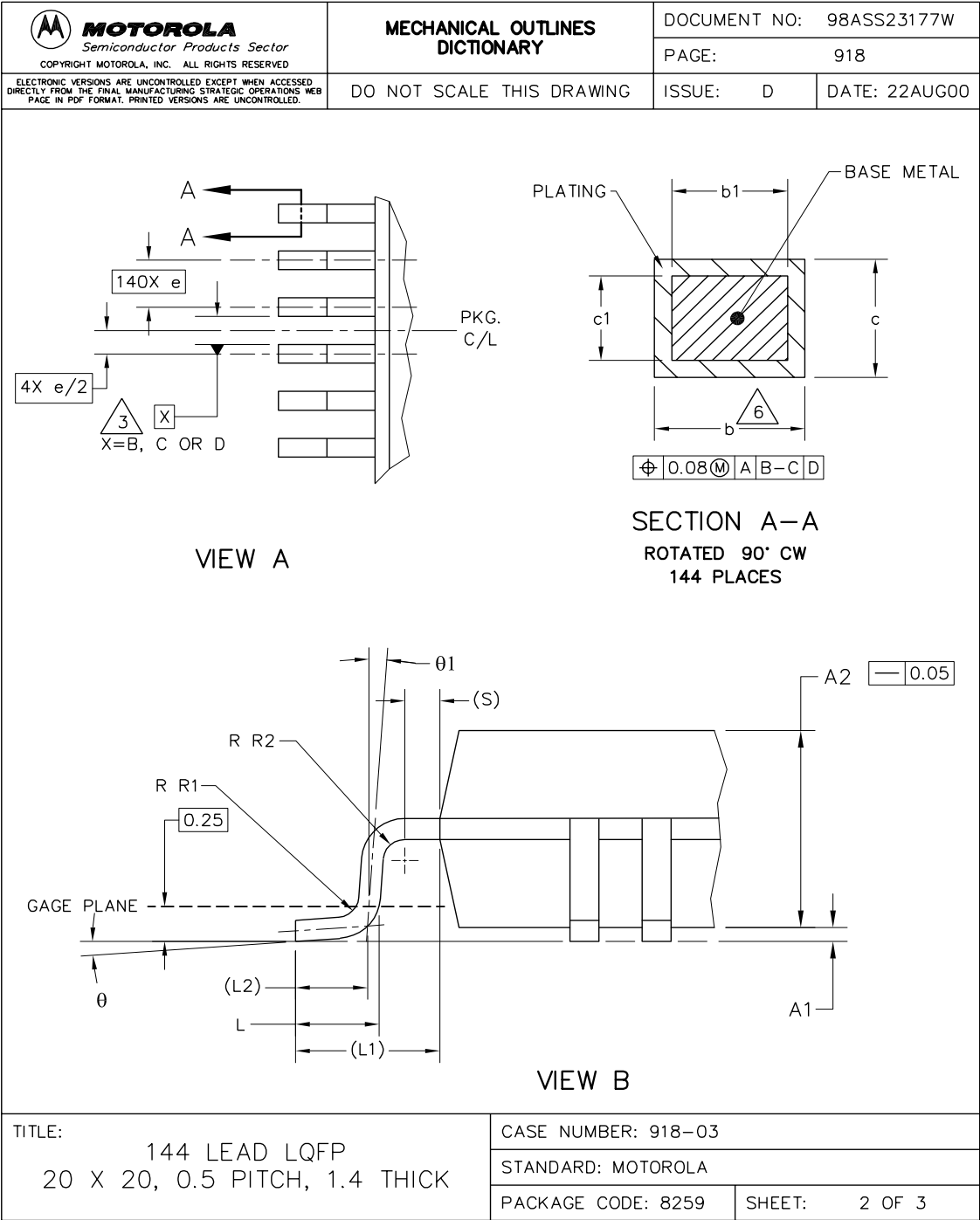
Figure 4-3 DSP56367 144-pin LQFP Package (2 of 3)
