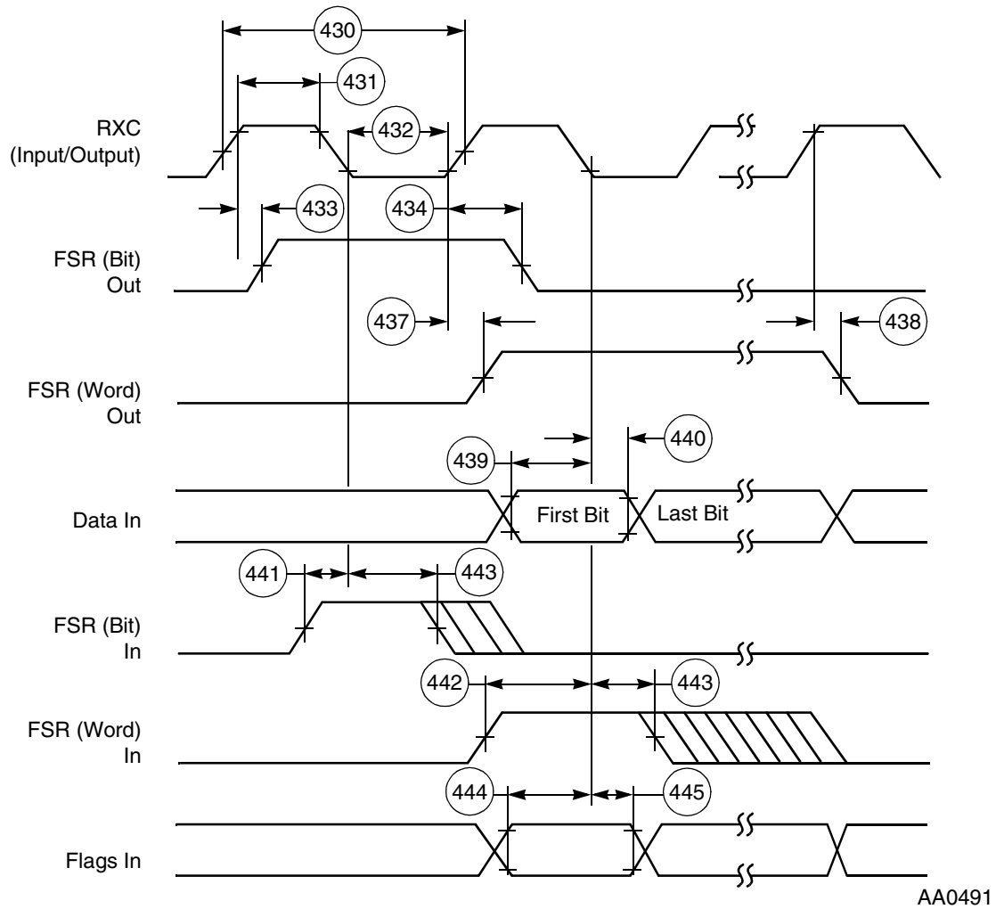
Figure 3-33 ESI Receiver Timing
