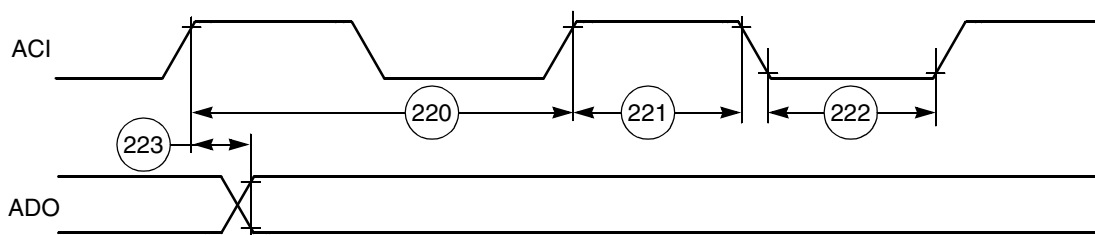
Figure 3-36 Digital Audio Transmitter Timing
