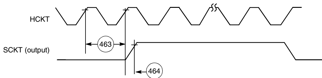
Figure 3-34 ESI HCKT Timing
