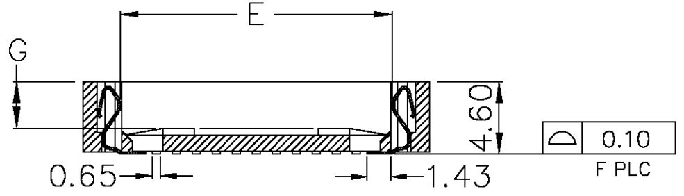
SECTION A-A SECTION B-B 44 POSITION SHOWN
