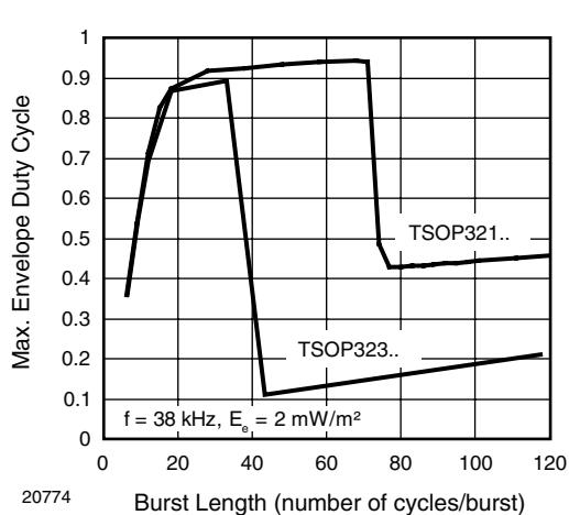
Fig. 9 - Maximum Envelope Duty Cycle vs. Burst Length
