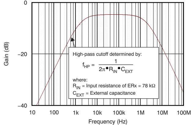
Figure 43. ERx Block Frequency Response
