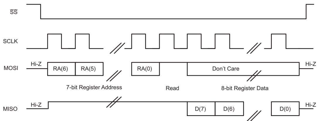
Figure 35. SPI Read
