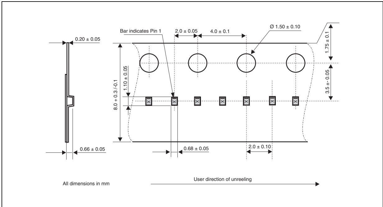
Figure 19. SOD882 tape and reel specifications
