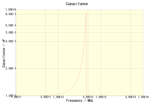
CKCA43C0G1H101K100AA
