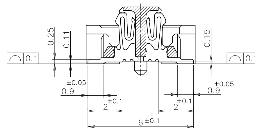
G-G (SIGNAL POSITION) (SCALE 8:1)
