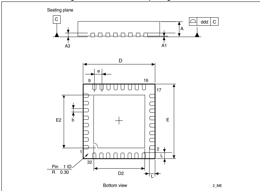
Figure 15. 32-lead VFQFPN package outline
