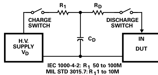
ELECTROSTATIC DISCHARGE TEST
