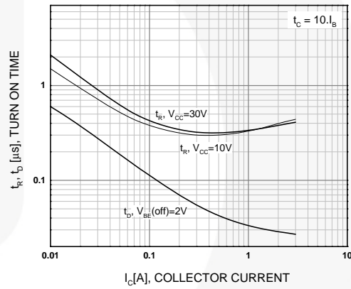
Figure 4. Turn-On Time
