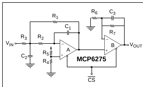
FIGURE 4-13: Second-Order Multiple Feedback Low-Pass Filter with an Extra Pole-Zero Pair.
