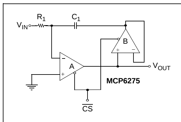
FIGURE 4-12: Integrator Circuit with Active Compensation.
