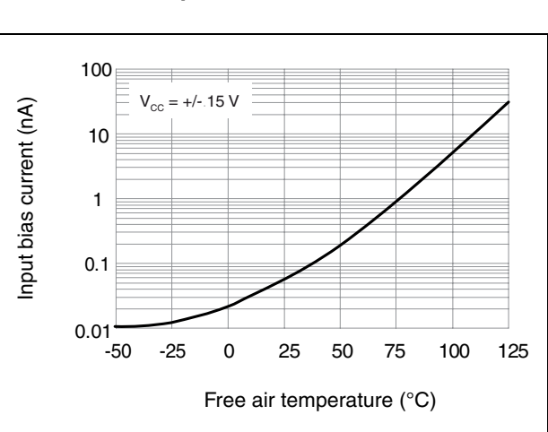
Figure 13. Input bias current versus free air temperature
