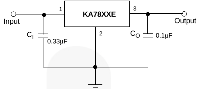
Figure 9. Fixed Output Regulator
