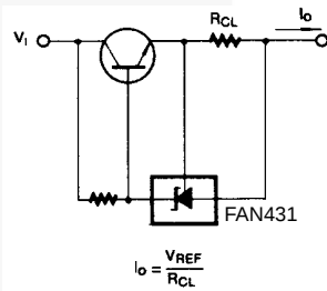
Figure 17. Current Limit or Current Source
