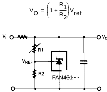
Figure 14. Shunt Regulator
