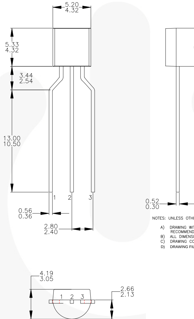
Figure 19. 3-Lead, TO-92, Molded, 0.200 in Line Spacing Lead Form
