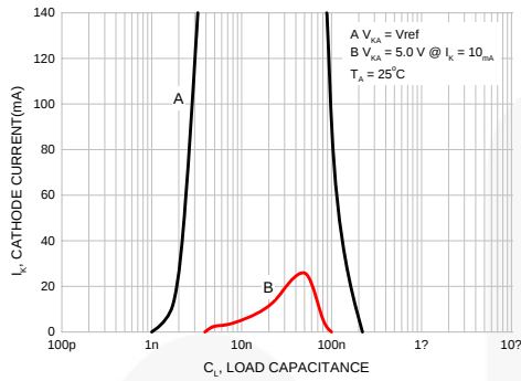
Figure11. Stability Boundary Conditions
