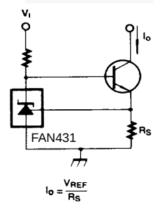
Figure 18. Constant-Current Sink
