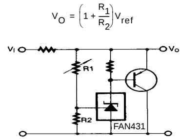
Figure 16. High-Current Shunt Regulator
