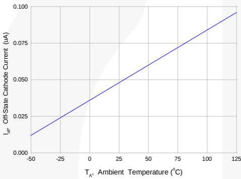
Figure 7. Ambient Temperature vs. OFF-State Cathode Current
