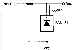
Figure 4. Test Circuit for I_{KA(OFF)}
