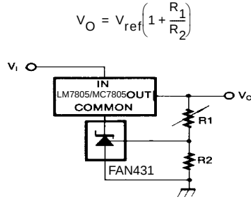
Figure 15. Output Control for Three-Terminal Fixed Regulator
