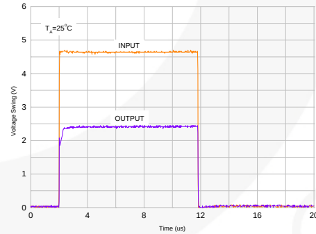
Figure 10. Pulse Response
