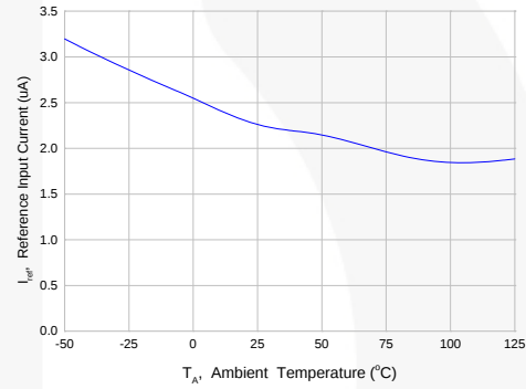
Figure 8. Ambient Temperature vs. Reference Input Current
