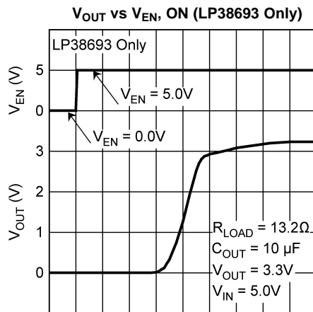
20 \mu\text{s}/\text{DIV} Figure 27.
