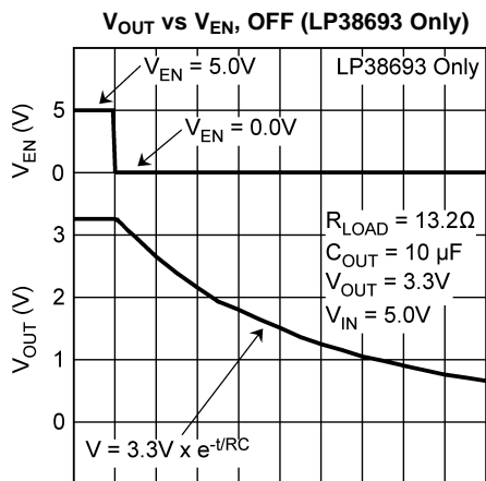
20 \mu\text{s}/\text{DIV} Figure 28.
