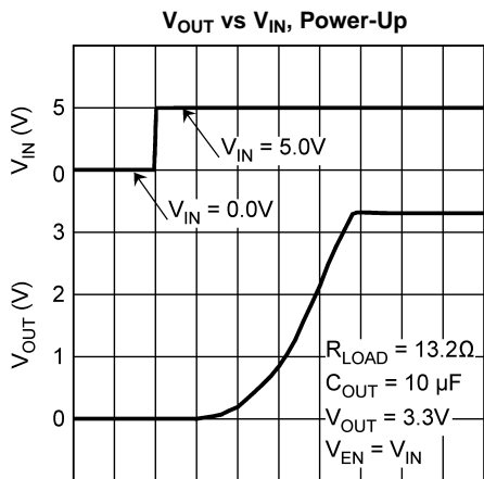
50 \mu\text{s}/\text{DIV} Figure 26.
