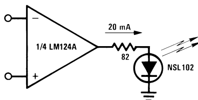
Figure 20. LED Driver
