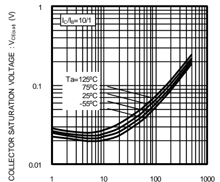
Fig6. Collector Saturation Voltage vs. Collector Current (I)
